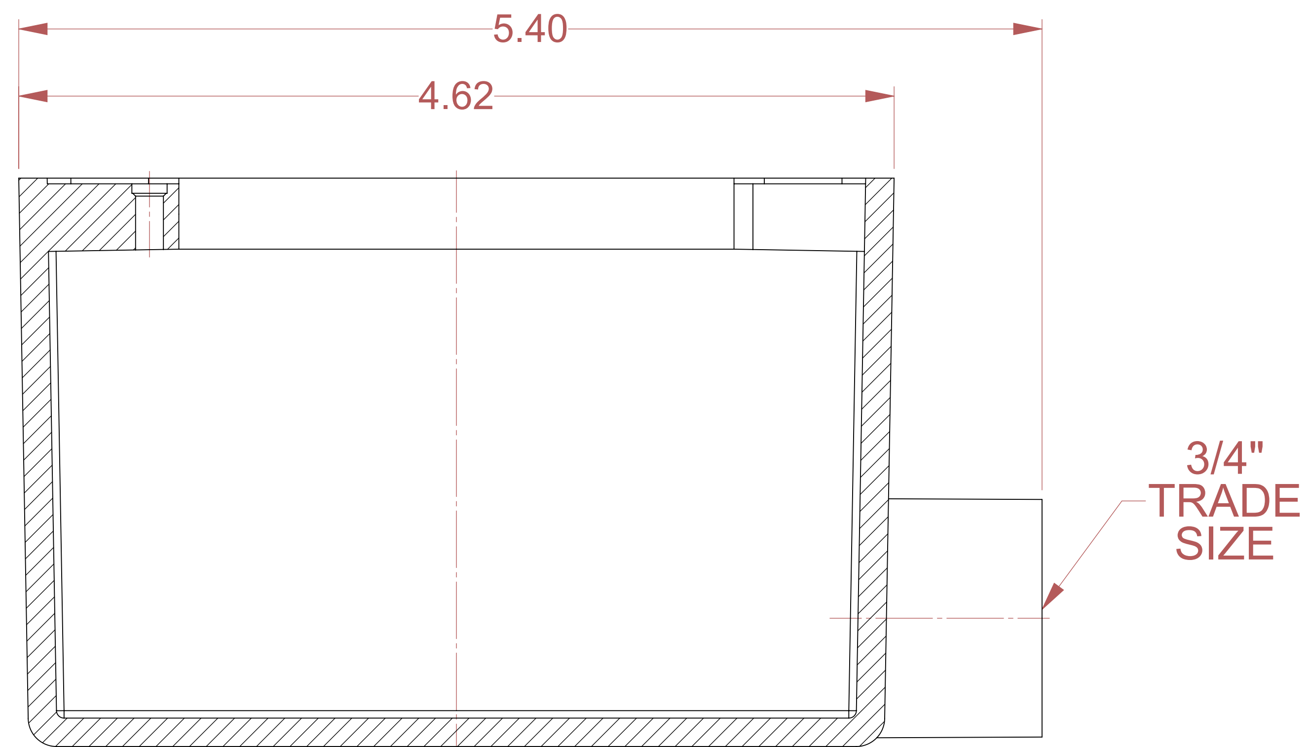
SECTION E-E
