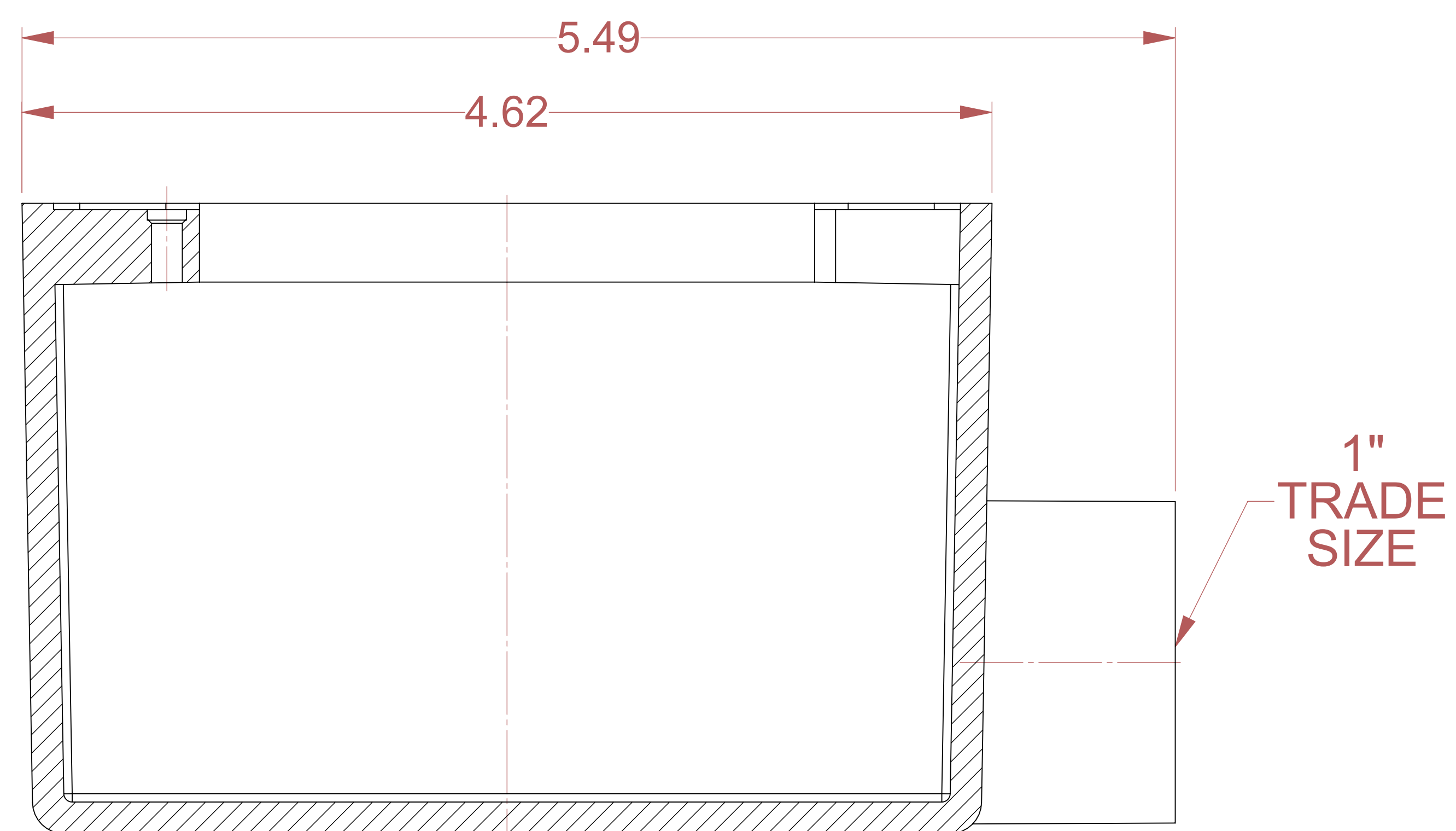
SECTION E-E
