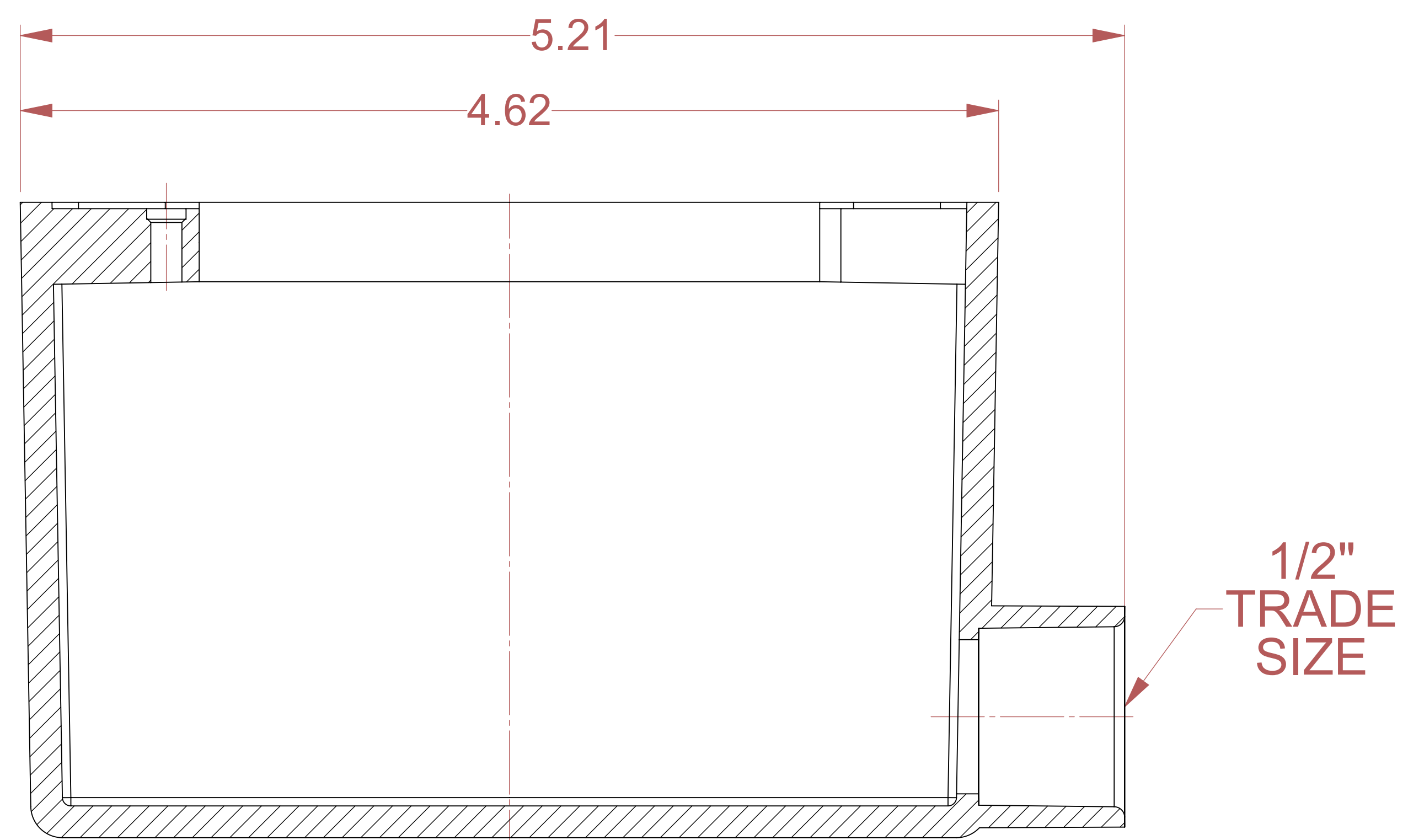
SECTION E-E
