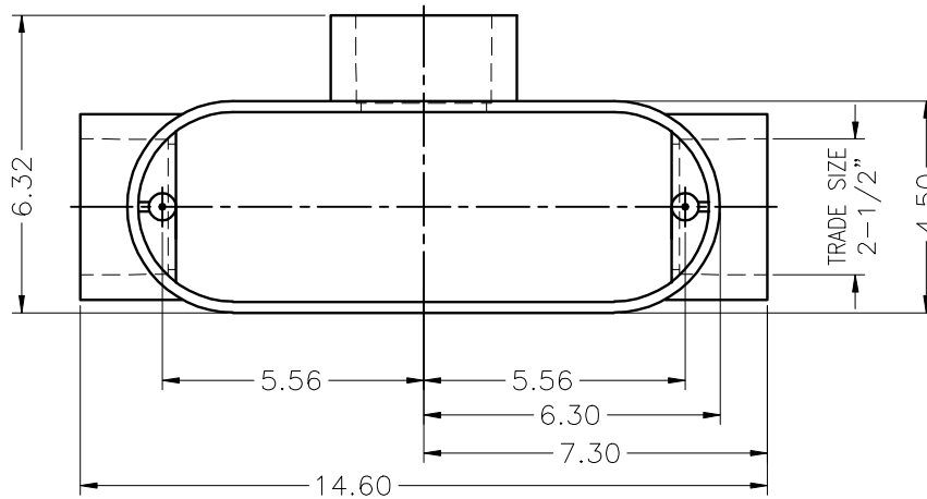
TOP VIEW W/O COVER
