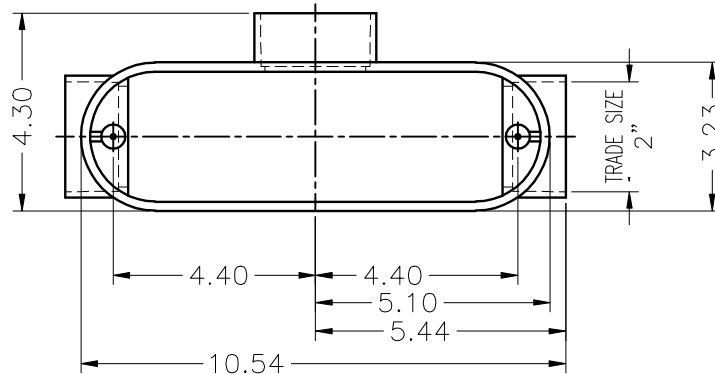
TOP VIEW W/O COVER
