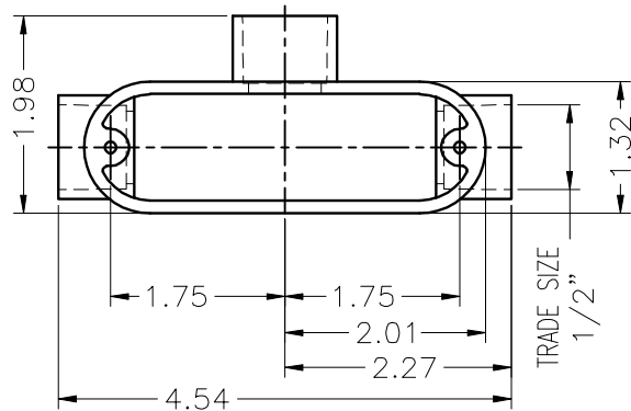
TOP VIEW W/O COVER
