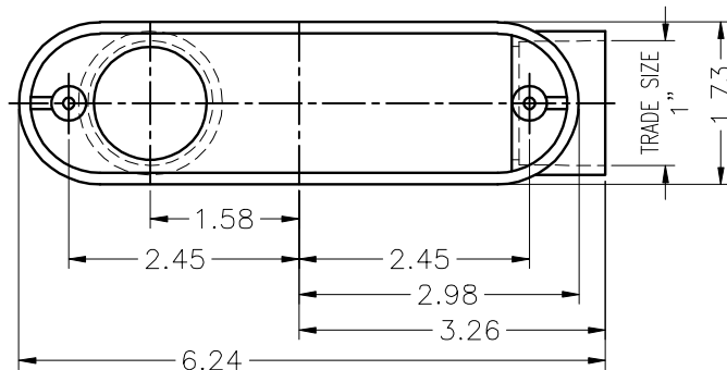
TOP VIEW W/O COVER
