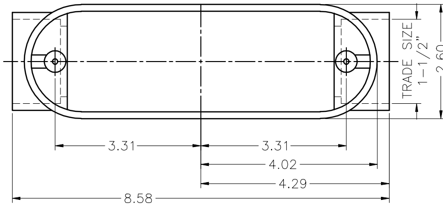
TOP VIEW W/O COVER
