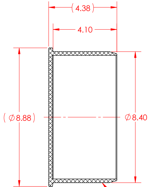
SECTION A-A 8" TRADE SIZE SDR35 SEWER SPIGOT
