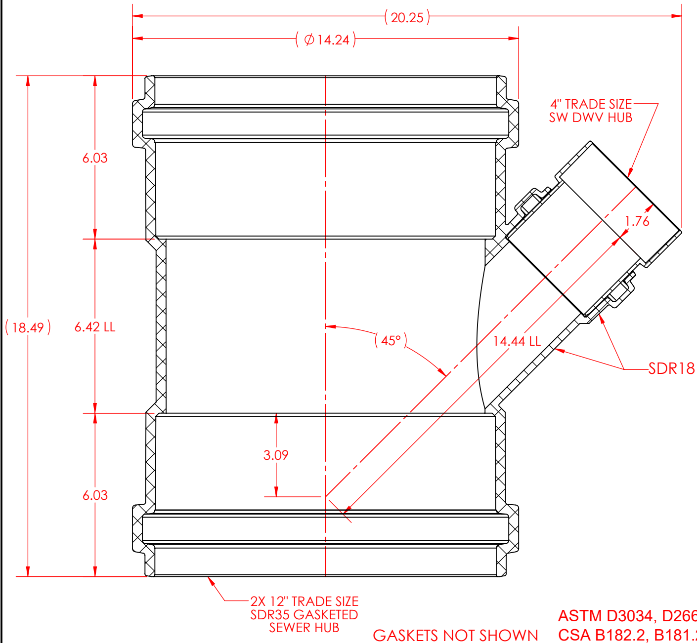
12" 45° WYE WITH 4" DWV BRANCH PVC SDR35 GASKETED SEWER 12"x 12"x 4" GxGxDWV H
